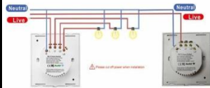
Two way control switch Diagram
