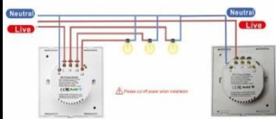
Two way control switch Diagram
