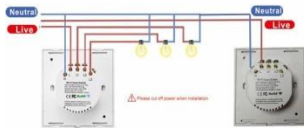
Two way control switch Diagram
